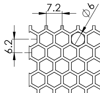
DETAIL A: 64% HEXAGON PERFORATED DOOR
