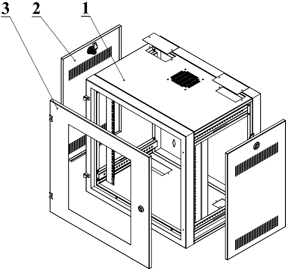
EXPLODE VIEW
