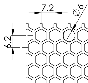
DETAIL A: 64% HEXAGON PERFORATED DOOR
