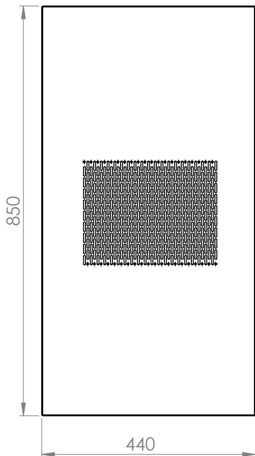
TOP VIEW
