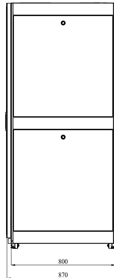
SIDE VIEW
