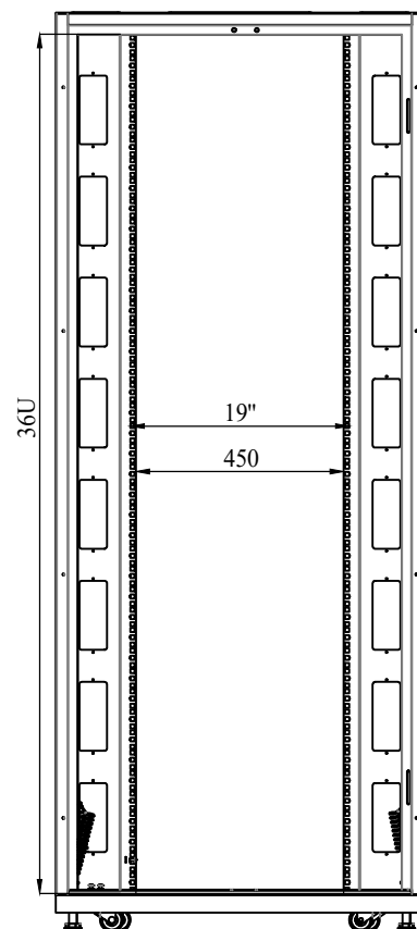
FRONT VIEW (REMOVED DOOR)
