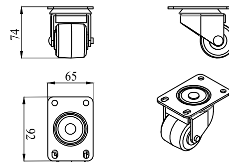
Caster
