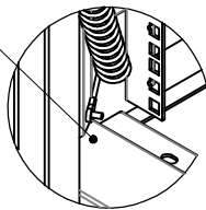
DETAIL A SCALE 1 : 5
