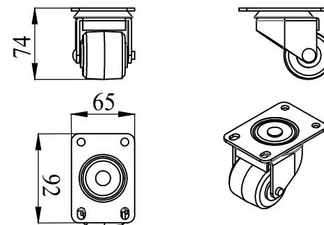
Caster
