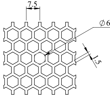
DETAIL A: HEXAGON >64% PERFORATED DOOR
