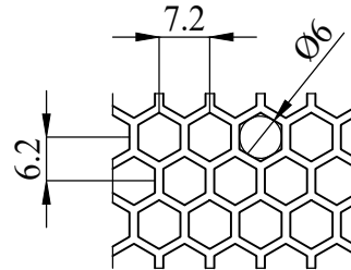
DETAIL A: 64% HEXAGON PERFORATED DOOR
