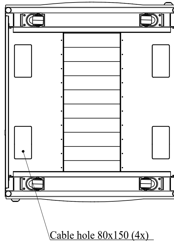
BOTTOM VIEW
