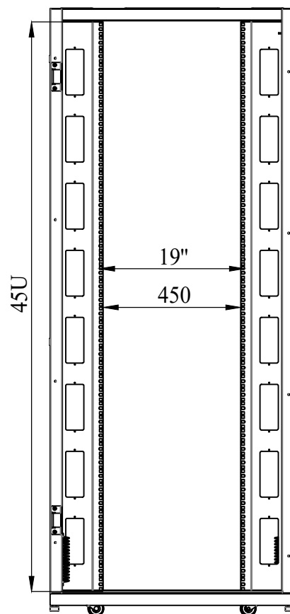
FRONT VIEW (REMOVED DOOR)
