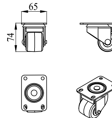
Caster
