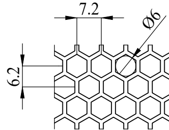
DETAIL A: 64% HEXAGON PERFORATED DOOR
