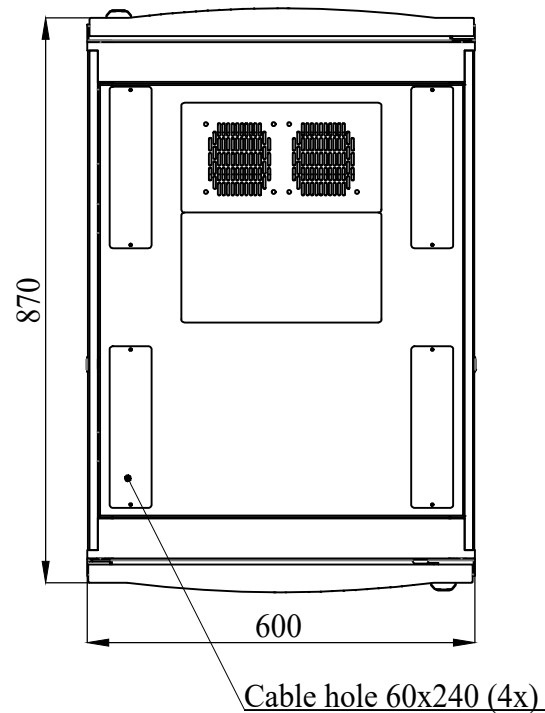
TOP VIEW
