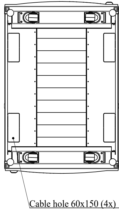
BOTTOM VIEW
