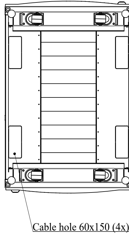
BOTTOM VIEW
