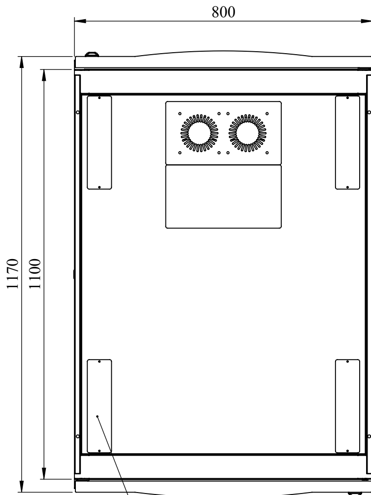
TOP VIEW
