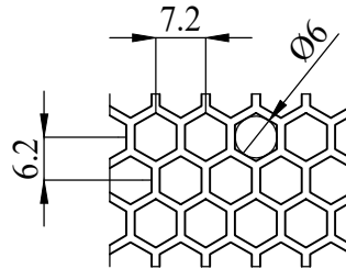
DETAIL A: >65% HEXAGON PERFORATED DOOR
