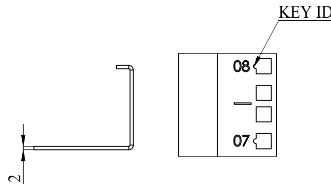
MOUNTING PROFILE WITH KEY ID&U-HIGH NUMBERING
