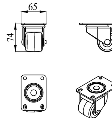
Caster
