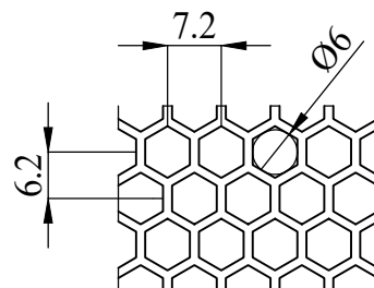
DETAIL A: >65% HEXAGON PERFORATED DOOR
