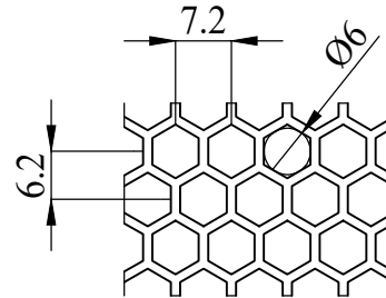
DETAIL A: >65% HEXAGON PERFORATED DOOR
