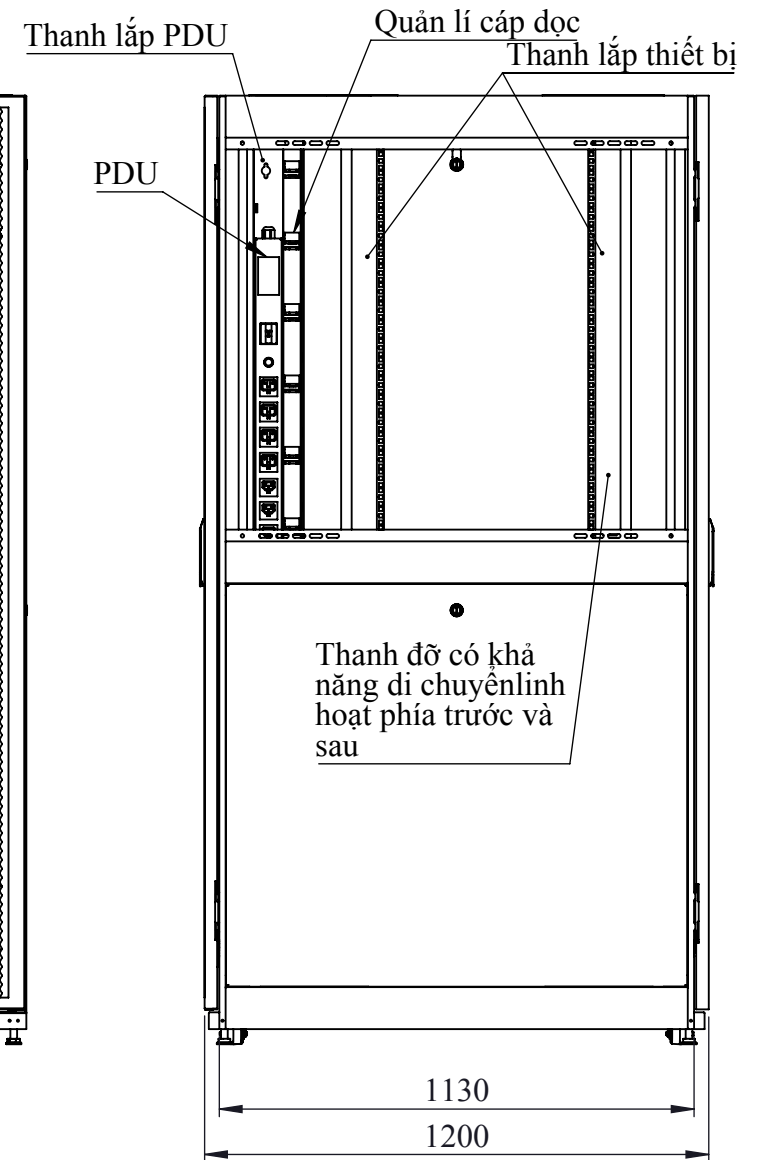
SIDE VIEW (REMOVED 1SIDE DOOR)
