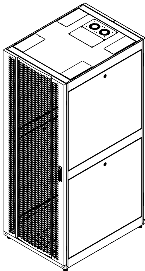
FRONT&RIGHT VIEW
