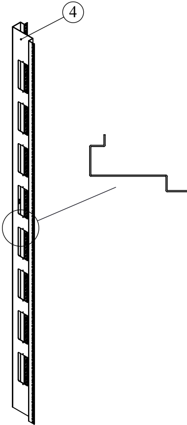
PROFILE BAR
