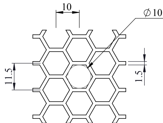
DETAIL A: HEXAGON >80% PERFORATED DOOR
